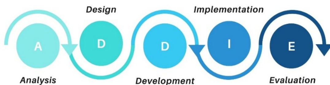
Fig. 1. ADDIE model
